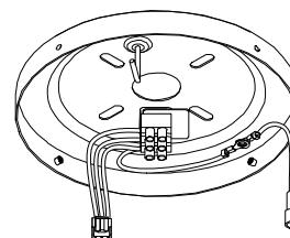
Ceiling bracket
